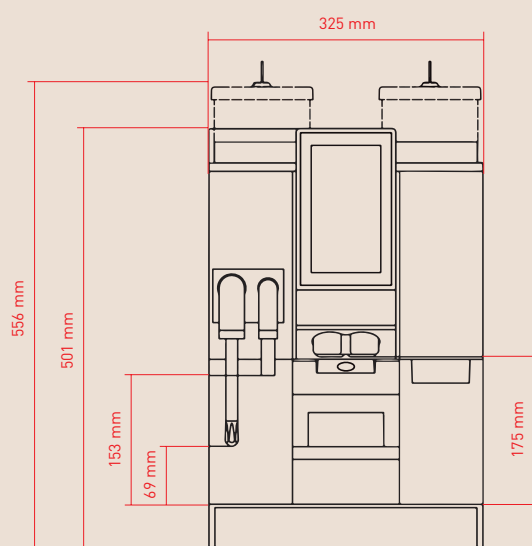
Schaerer Coffee Club Depth: 570 mm
